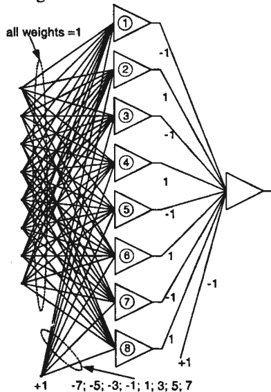
Fig. 23. Parity-8 problem with feedforward bipolar neural network with one hidden layer.
