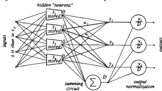
Fig. 19. RBF - Radial basis function networks.
