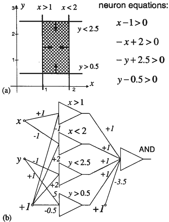
Fig. 11. Separation of the rectangular area on a two dimensional space (a) and desired neural network to fulfill this task (b).
