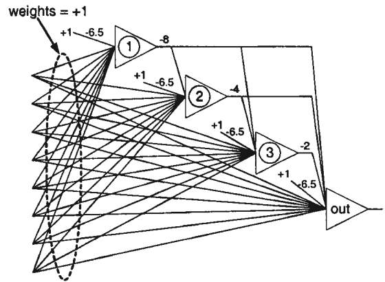
Fig. 25. Bipolar implementation of a fully connected cascade neural network for the parity-8 problem.
