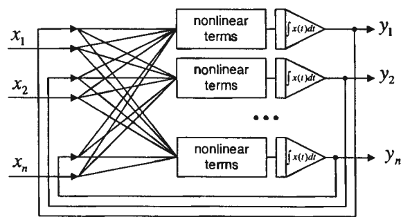
Fig. 1. Block diagram of nonlinear system derived from a set of state variable equations.
