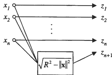
Fig. 21. Networks with increased dimensionality.
