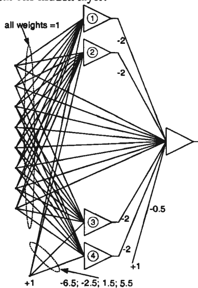
Fig. 24. Fully-connected layered bipolar neural network with one hidden layer for the parity-8 problem.
