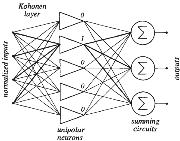
Fig. 16. Counterpropagation networks.
