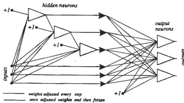
Fig. 18. Cascade correlation architecture.
